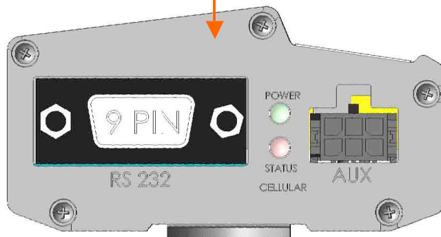
Pinbelegung RS-232 D-Type 9 pin female RS232
